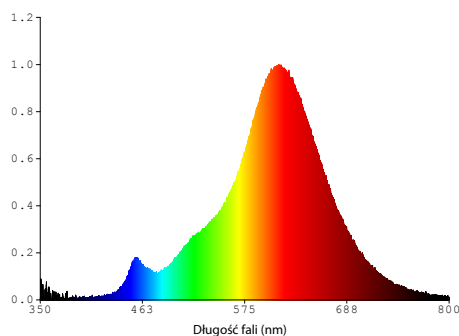
LEDSTAR AMBER C35, 5W, 2200K
